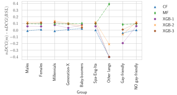
Figure 4: nDCG difference between ML-models and BSL.
